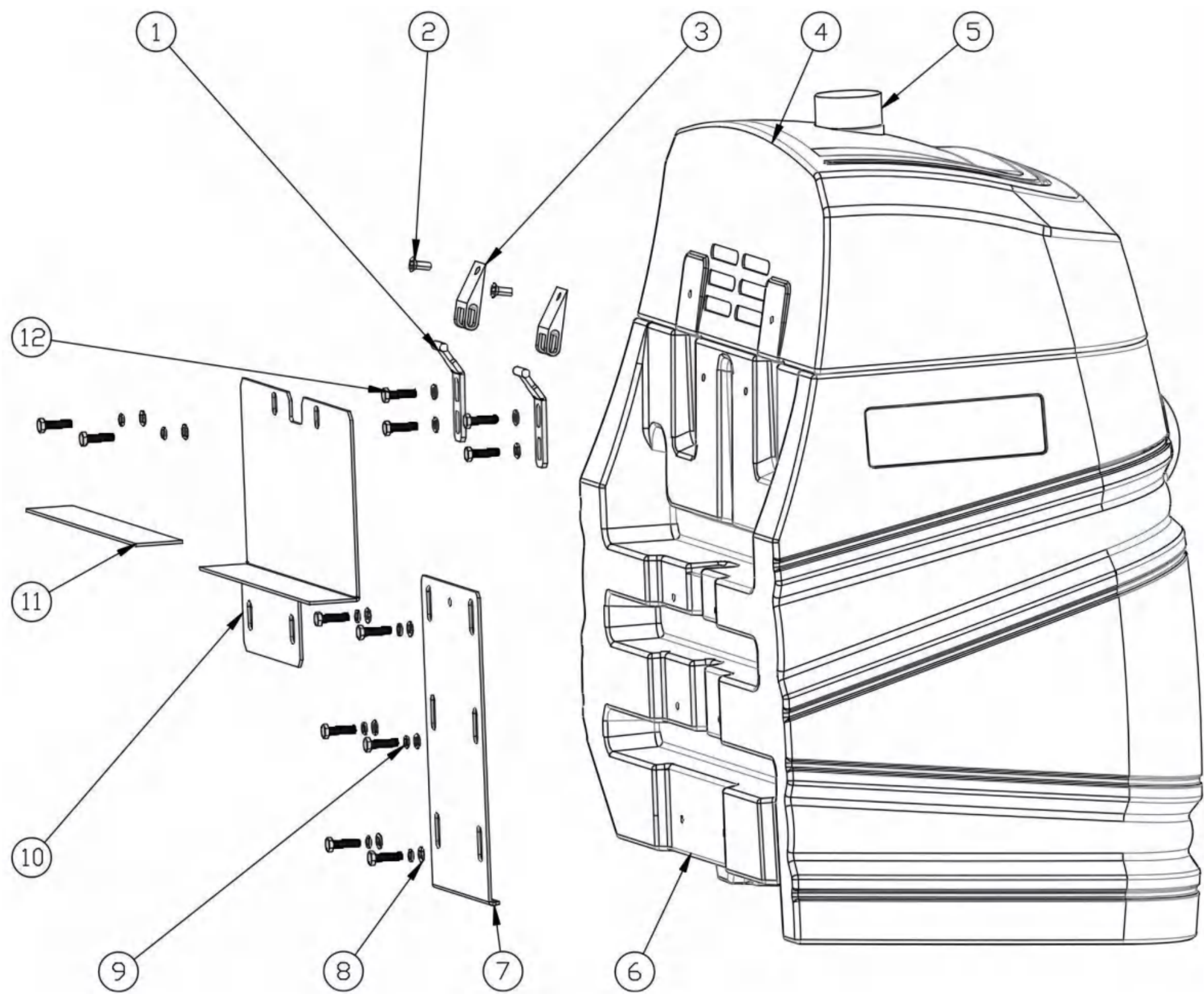
Fig. 2 -RECOVERY TANK GROUP
