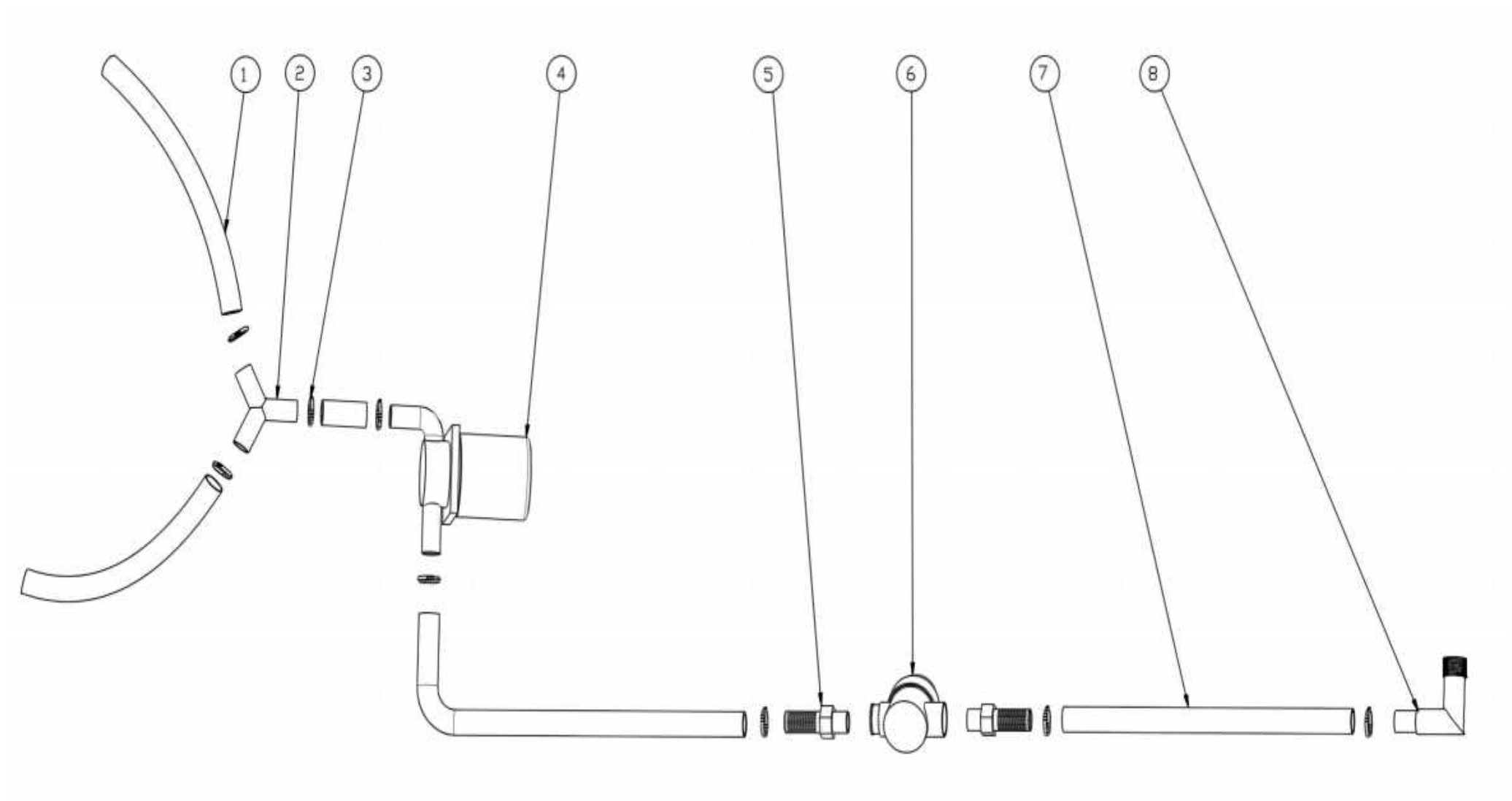
Fig. 10 -HOSE GROUP
