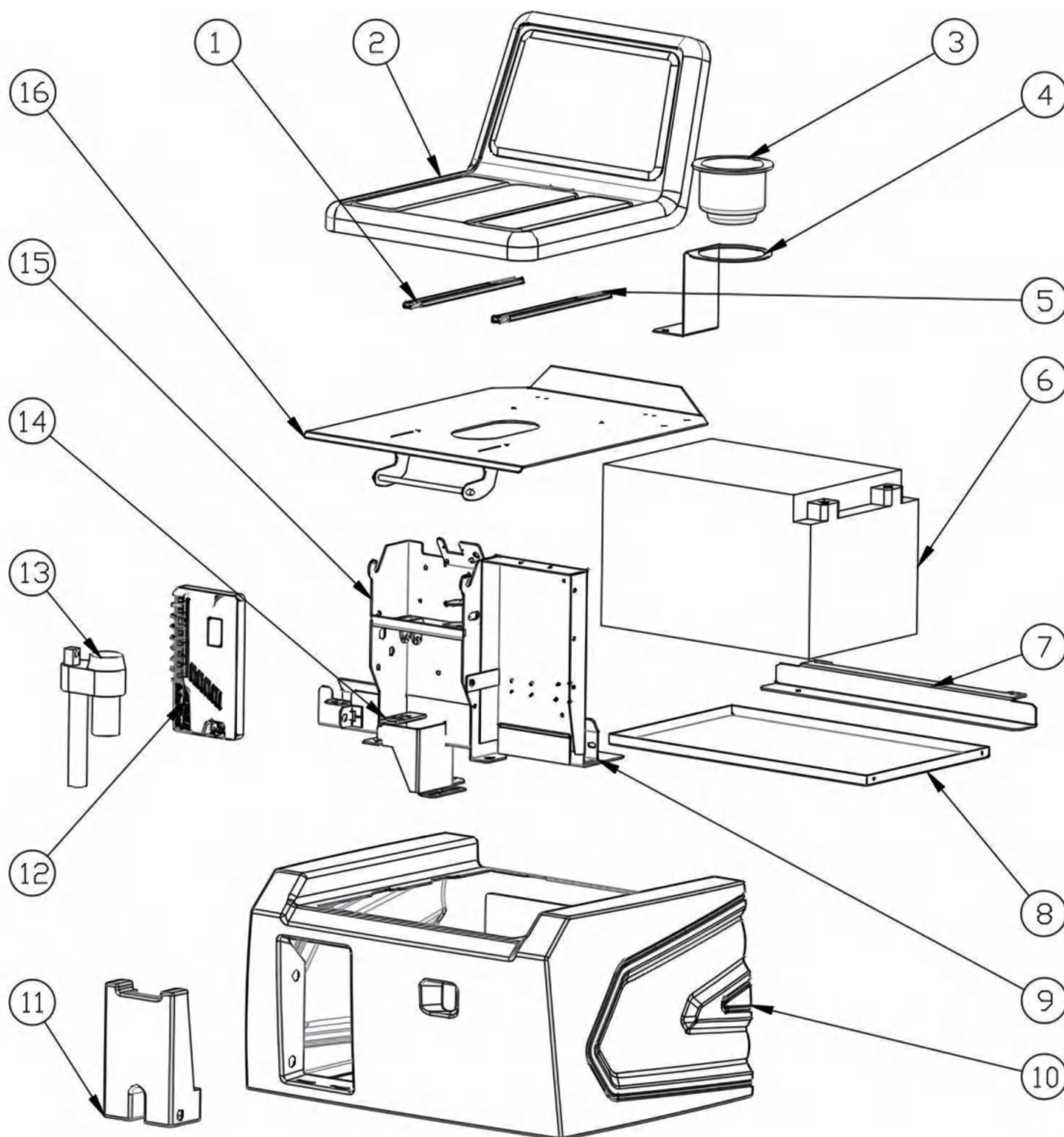
Fig. 5 -SEAT GROUP
