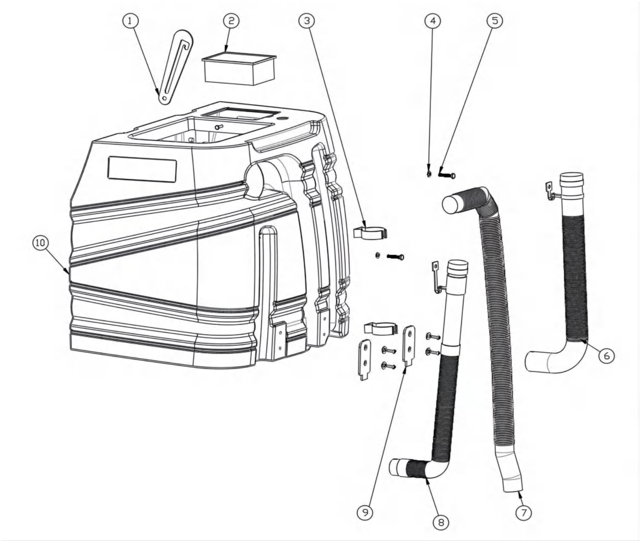
Fig. 9 -TANKS DRAIN GROUP
